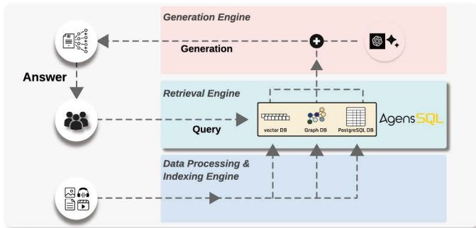
< Graph RAG Architecture >
